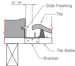
Side Detail
