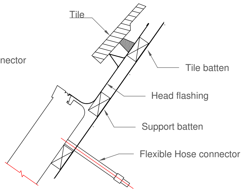
SECTION 2-2
