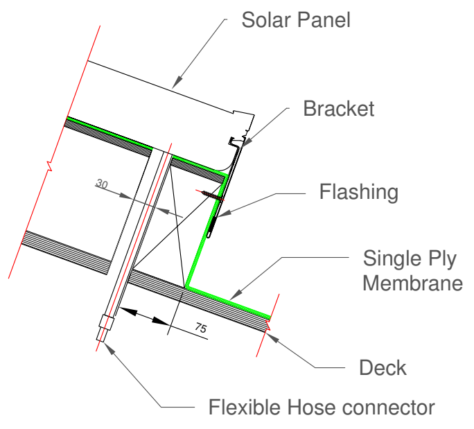
SECTION 1-1
