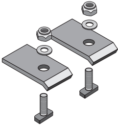
10115 Panel clamp set for VHL20
