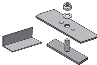
10117 Clamp kit & jig for each additional VHL20
